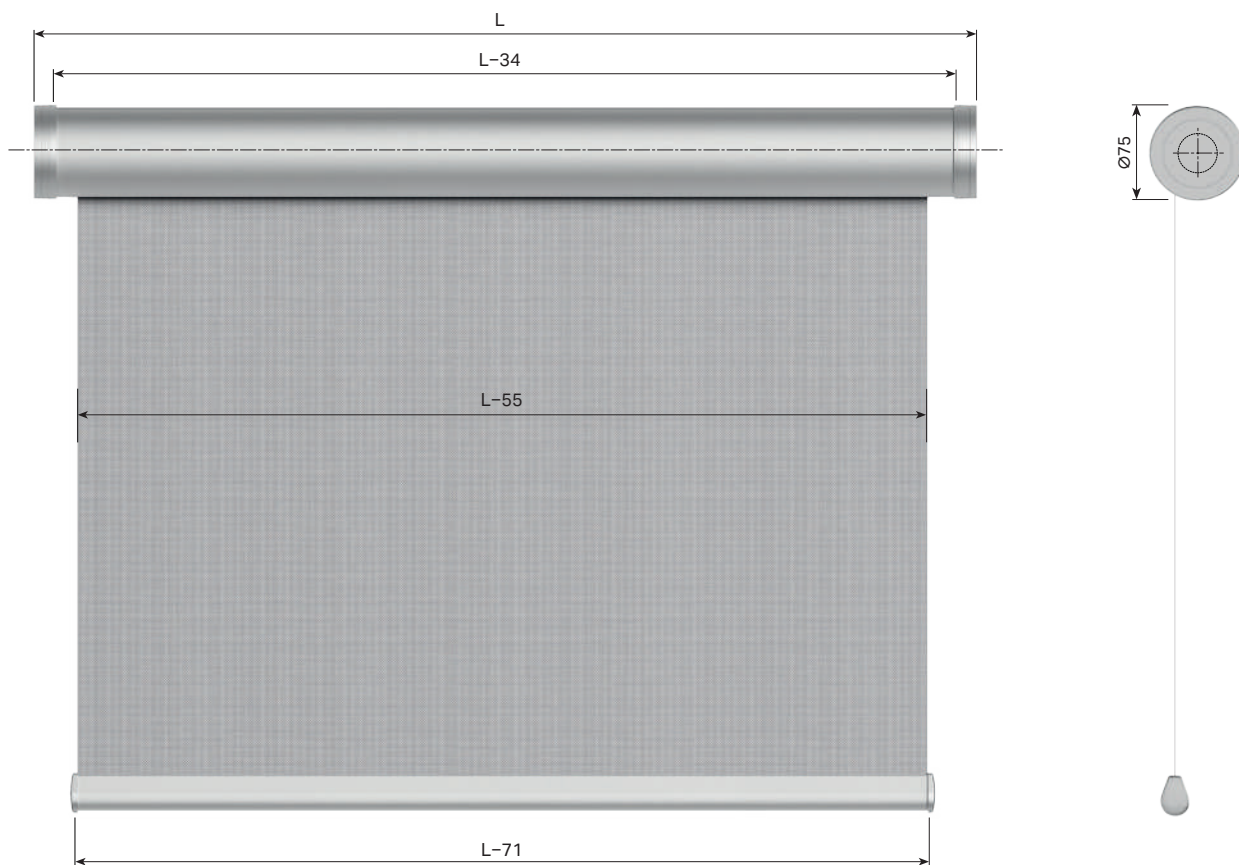
ROLLBOX 475
